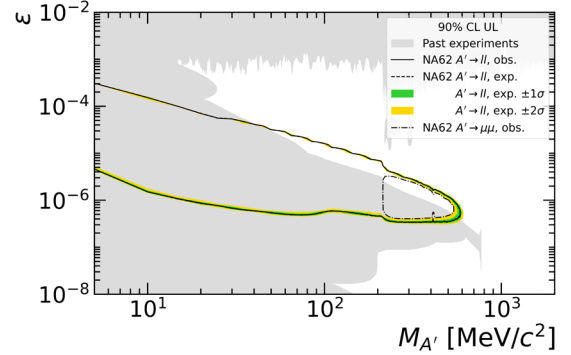
Figure 10: Exclusion contour obtained by the combination of A' \rightarrow e^+e^- and A' \rightarrow \mu^+\mu^- searches. The same color conventions as in are Figure 9 used.
