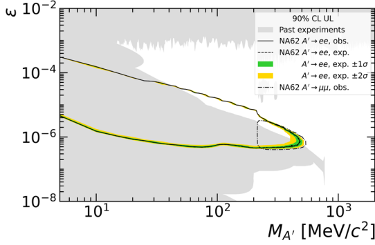
Figure 9: Exclusion contour obtained by the A' \rightarrow e^+e^- search. The same color conventions as in Error! Reference source not found. are used. The dot-dashed contour is the one obtained by NA62 in the A' \rightarrow \mu^+\mu^- search
