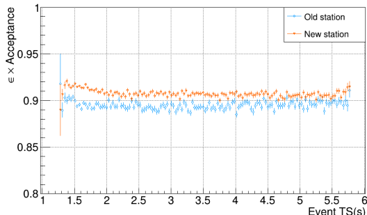
Figure 7: Effective efficiency by station, blue for old and orange for new, as function of time during a burst
