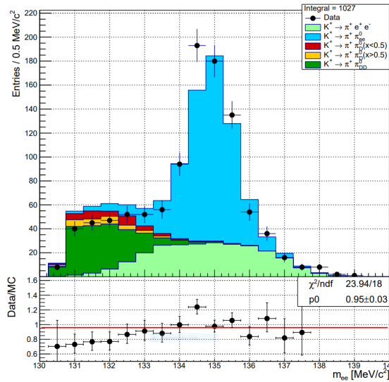
Figure 11: Data – Monte Carlo comparison of the reconstructed mass of the e^+e^- pair using the updated selection. The data sample contains the runs collected in 2017 and 2018.
